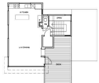
3RD FLOOR PLAN
