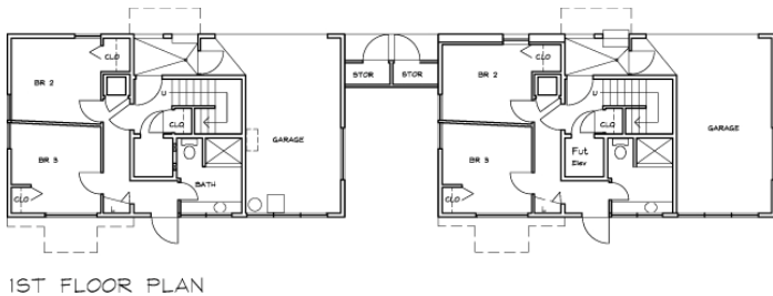
1ST FLOOR PLAN
